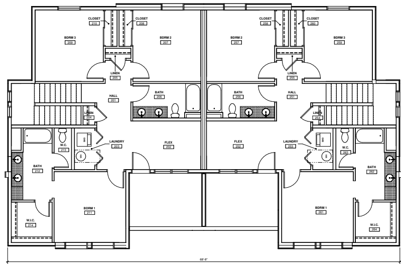
SECOND FLOOR PLAN ② SCALE: 1/4" = 1'-0"
